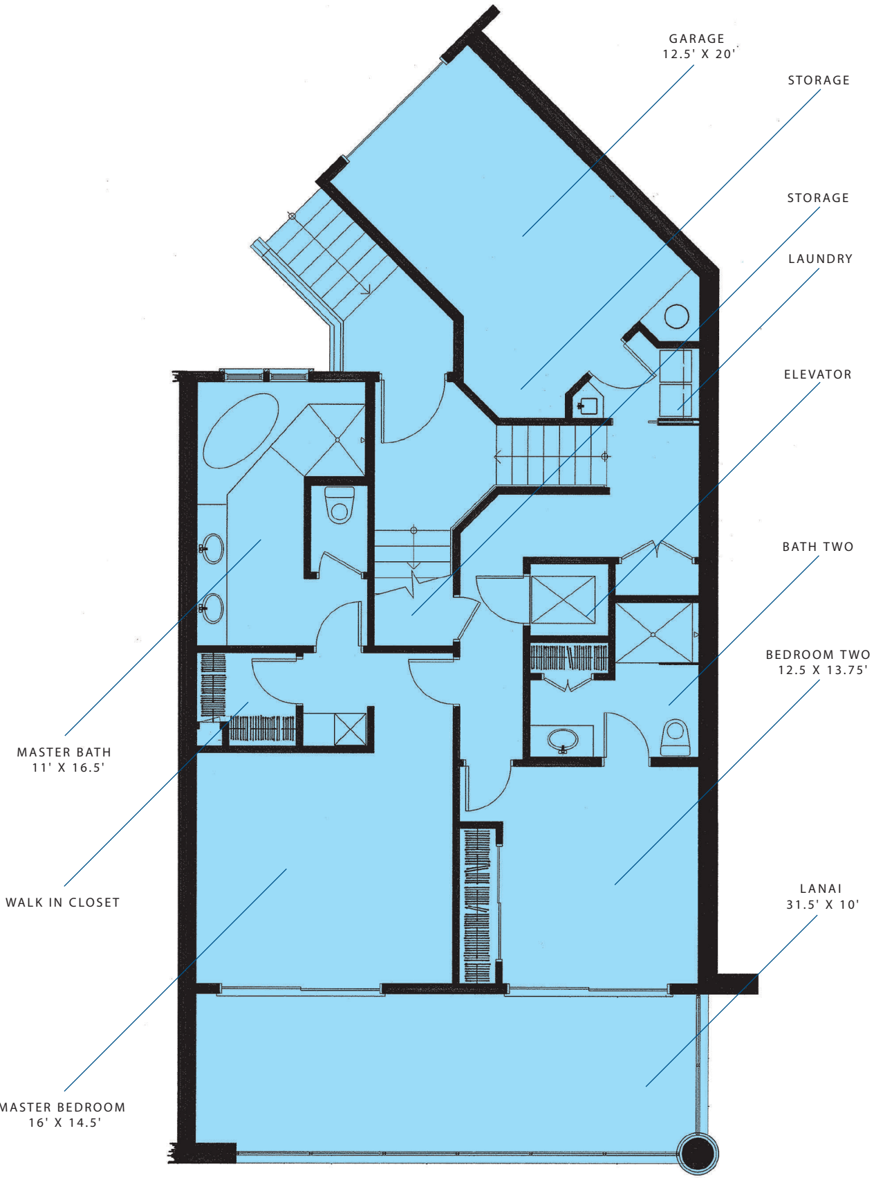
FIRST FLOOR
